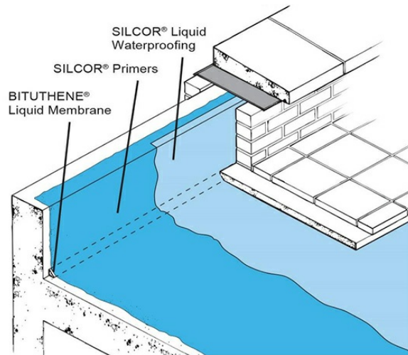
Details shown are typical illustrations only and not working drawings. For assistance with working drawings and additional technical advice please contact GCP Technical Services.
